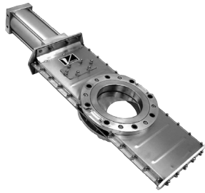
Pneumatic knife gate
