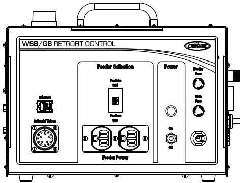
01 WSB/GB Retrofit Control
