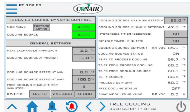
Figure 50 User Setup – Free Cooling Dynamic Isolated Source
