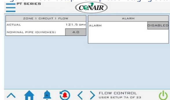
Figure 41 User Setup – Compressor Staging Setup
