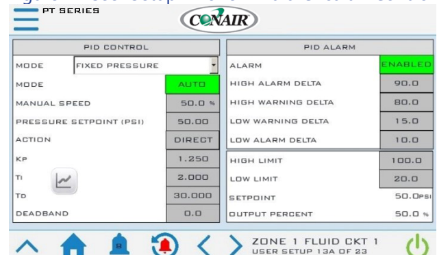
Figure 47 User Setup – Zone X Fluid Circuit X Control
