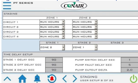
Figure 42 User Setup – Stage Order Setup
