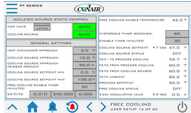
Figure 49 User Setup – Free Cooling Static Isolated Source
