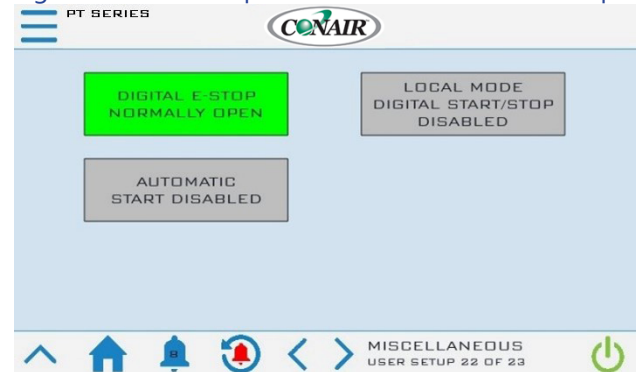
Figure 58 User Setup – Miscellaneous Control Setup S
