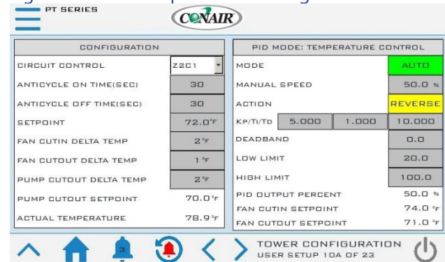
Figure 44 User Setup – Tower Configuration
