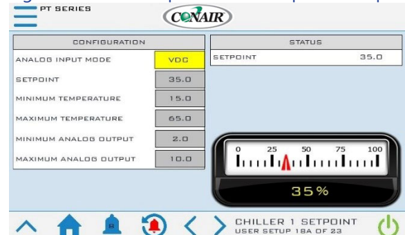
Figure 55 User Setup – Remote Setpoint Setup
