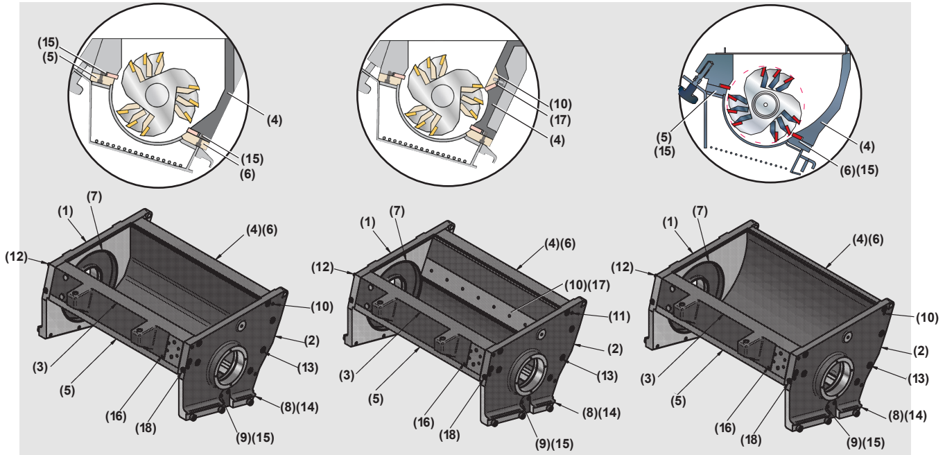
(A) = CUTTER HOUSING 1ST "TANGENTIAL" 3-68108-C01, 3-68182-C01, 3-68104-C01, 3-68185-C01, 3-068100-C01, 3-68179-C01, 3-68112-C01, 3-68188-C01
