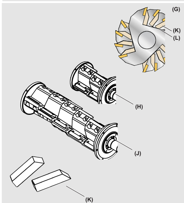
(G) = 3-blade staggered rotor (H) = 3-blade staggered rotor, NCF-810 (J) = 3-blade staggered rotor, NCF-824 (K) = Rotating knife, 3-blade staggered rotor (L) = Support rule, 3-blade staggered rotor
