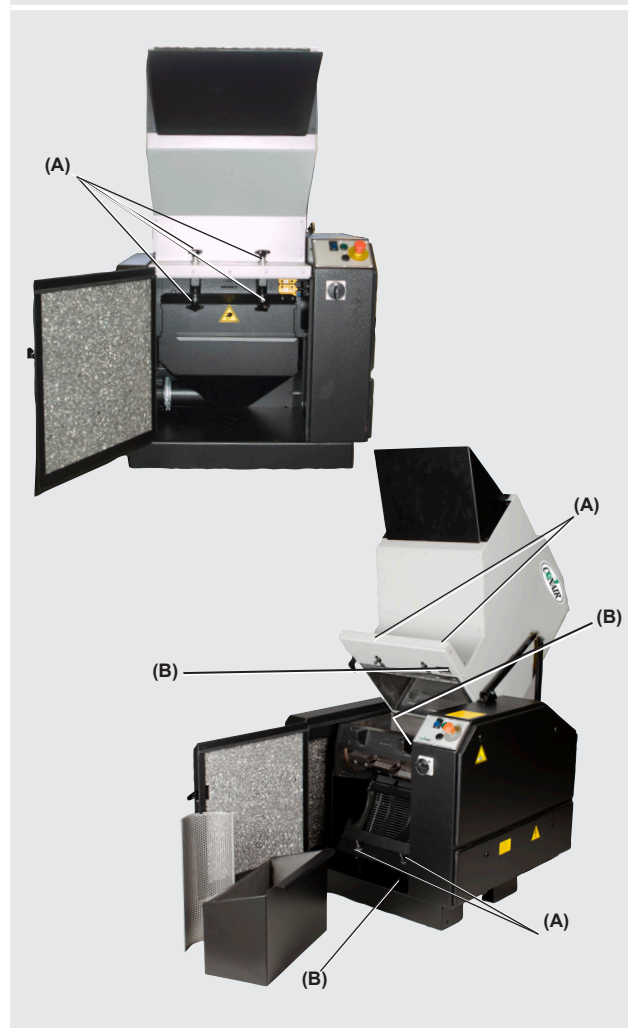
(A) = Star knob (B) = Safety sensor
