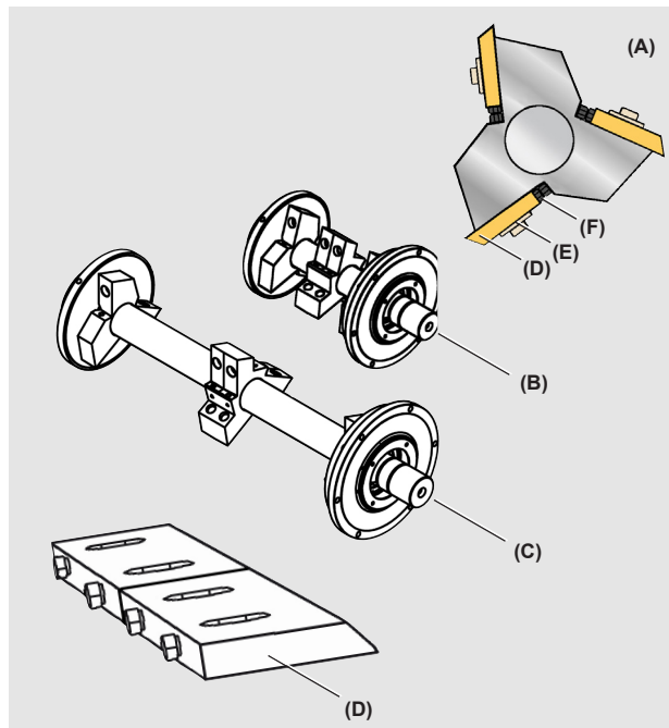
(A) = 3-blade open rotor (B) = 3-blade open rotor, NCF-810 (C) = 3-blade open rotor, NCF-824 (D) = Rotating knife, 3-blade open rotor (E) = Washer, 3-blade open rotor (F) = Adjusting screw, 3-blade rotor
