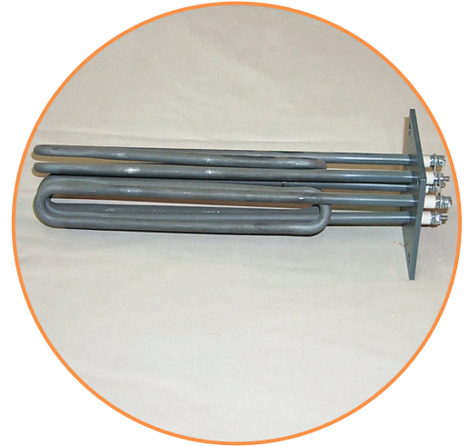
Heating Elements for Dryers - D-30 Dryer
